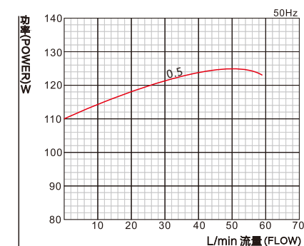
功率—流量曲线图 Power - flow curve
