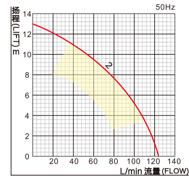
扬程—流量曲线图 Lift - flow curve
