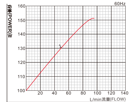
功率—流量曲线图 Power - flow curve
