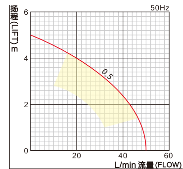
扬程—流量曲线图 Lift - flow curve
