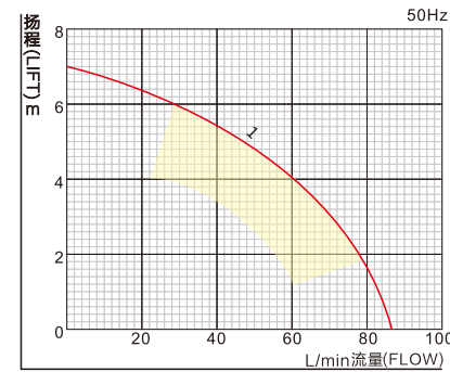
扬程—流量曲线图 Lift - flow curve
